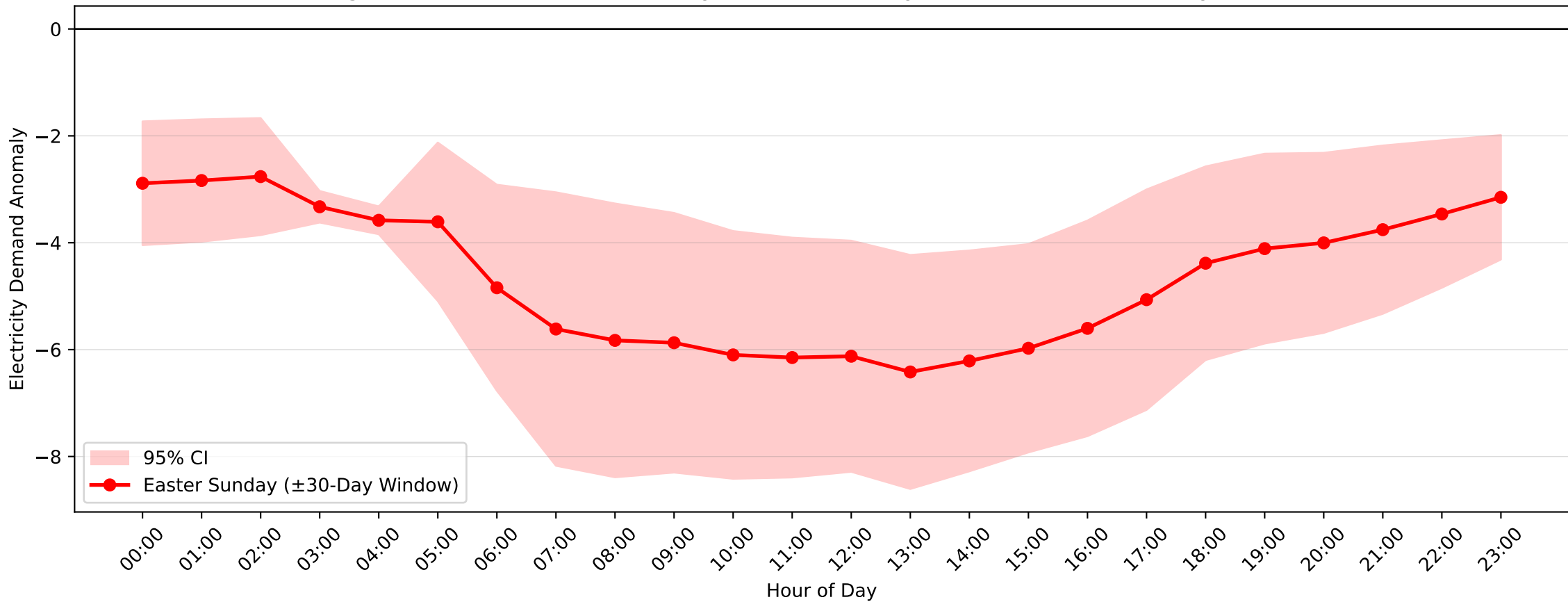
Leightonfield Demand Anomaly: Easter Sunday (2004-2017, \pm 30 -Day Window)
